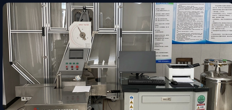
Automated Charpy impact tester with cooling unit
