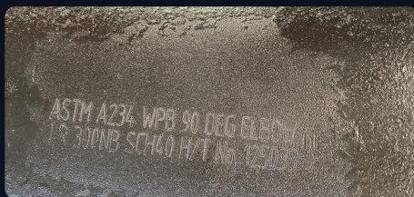
Heat-number marking, traceable to MTC
